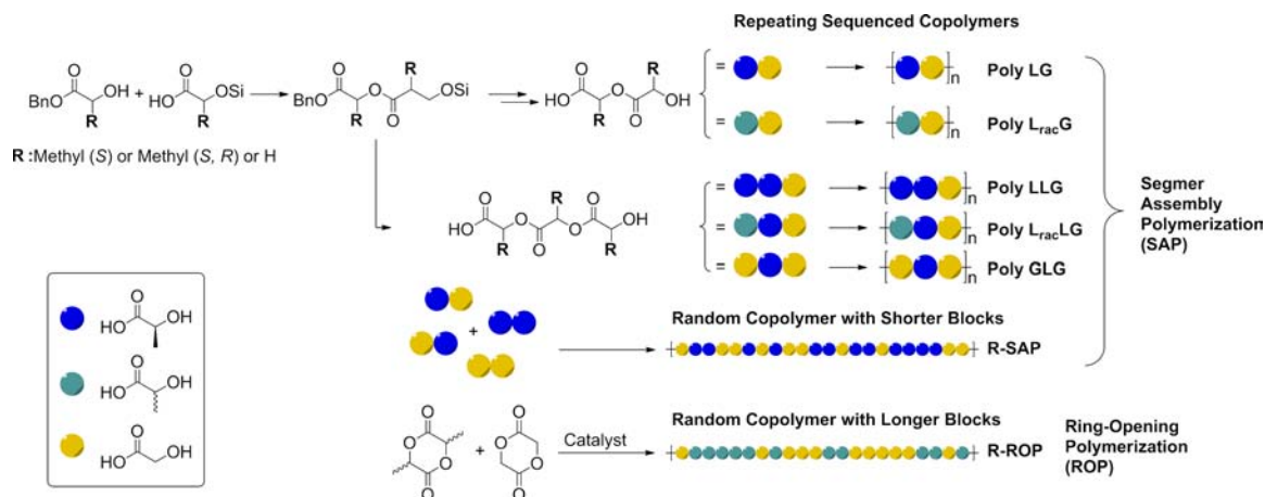
Figure 2. (Top) Segmer assembly polymerization (SAP) used to prepare repeating sequence copolymers and a random copolymer of poly(lactic-co-glycolic acid). (Bottom) Ring-opening polymerization (ROP) used to prepare a random copolymer.
