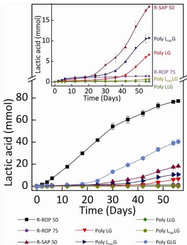
Figure 5. Lactic acid release rate as a function of hydrolytic degradation time. Inset shows the magnified plots of PLGAs with lower lactic acid release rates.
