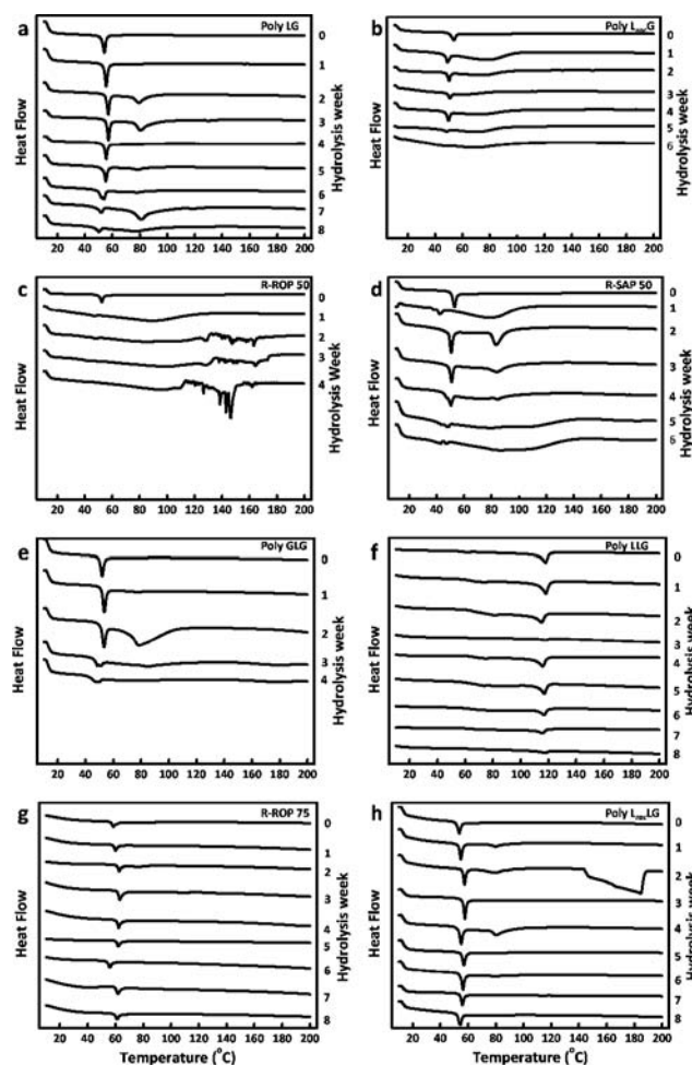
Figure 6. DSC thermograms of PLGAs in the hydrolysis study. (a) Poly LG ; (b) Poly L rac G ; (c) R-ROP 50 ; (d) R-SAP 50 ; (e) Poly GLG ; (f) Poly LLG ; (g) R-ROP 75 ; (h) Poly L rac LG (large feature at >160 °C week 2 is not related to the sample). For rapidly degrading samples, DSCs could not be obtained for the entire 8-week-period due to the decrease in material available.
