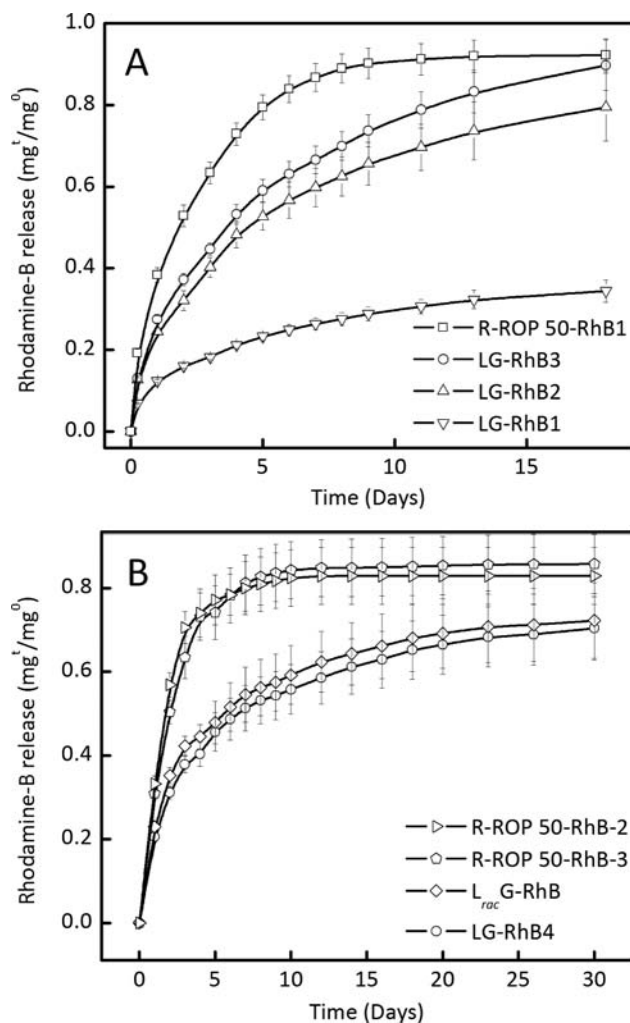
Figure 7. Release of RhB from PLGA microparticles immersed in a pH 7.4 buffer at 37 °C: (A) 18-day study focusing on particle loading; (B) 30-day study focusing on sequence dependence of release. Error bar showing standard deviation is obtained from four replicates.
