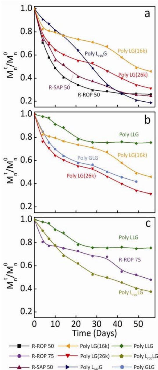
Figure 3. Molecular weight loss as a function of hydrolytic degradation time for the repeating sequenced and random sequenced PLGAs: (a) comparison of all polymers with a 50:50 LG ratio; (b) comparison of polymers with varying L:G ratios; (c) comparison of LLG polymers with varying stereochemistries.
