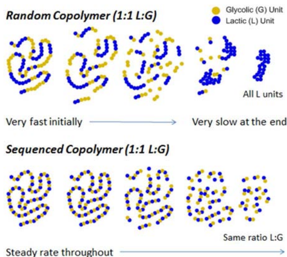
Figure 8. Proposed difference in hydrolysis pattern for random and sequenced PLGA copolymers with the same L:G ratio.
