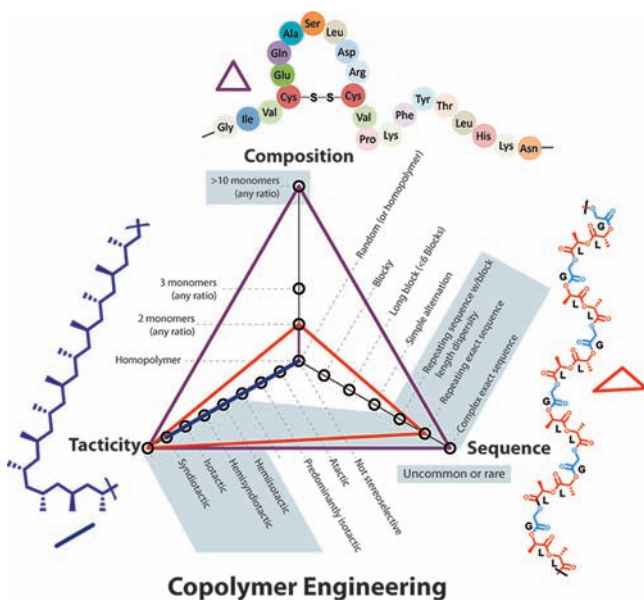
Figure 1. Radar plot of copolymer characteristics: composition (vertical axis), sequence (right axis), and stereochemical control (left axis). Repeating sequence exact tacticity PLGAs (red) exhibit levels of sequence and stereochemical control near to those expressed in proteins (gray). Related synthetic polymers are plotted for comparison.
