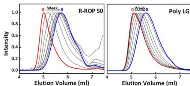
Figure 4. SEC traces for random copolymer (left) and alternating sequence PLGA copolymers (right) with 1:1 ratios of lactic and glycolic acids.
